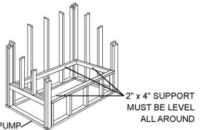
ALTERNATIVE CABINET CONSTRUCTION
