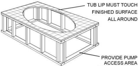
TYPICAL CABINET CONSTRUCTION
