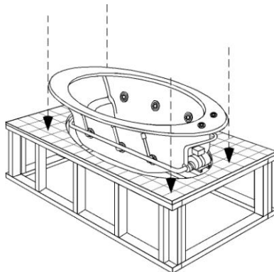
ALTERNATIVE CABINET CONSTRUCTION
